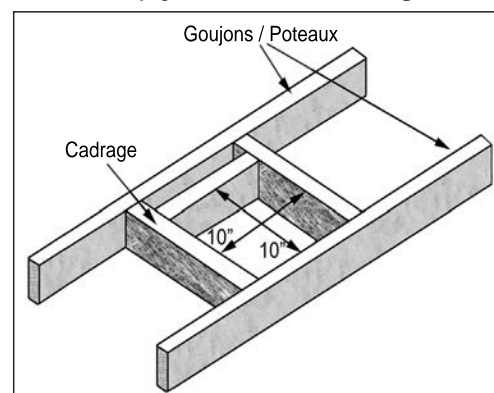
Figure 22. Vent Framing For Wall or Ceiling
