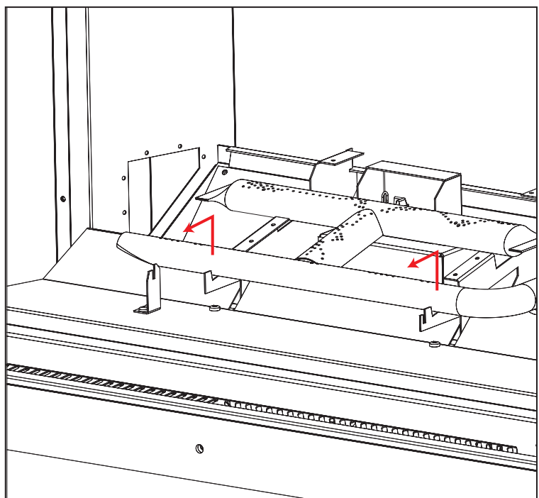
Figure 11. Removing Burner
