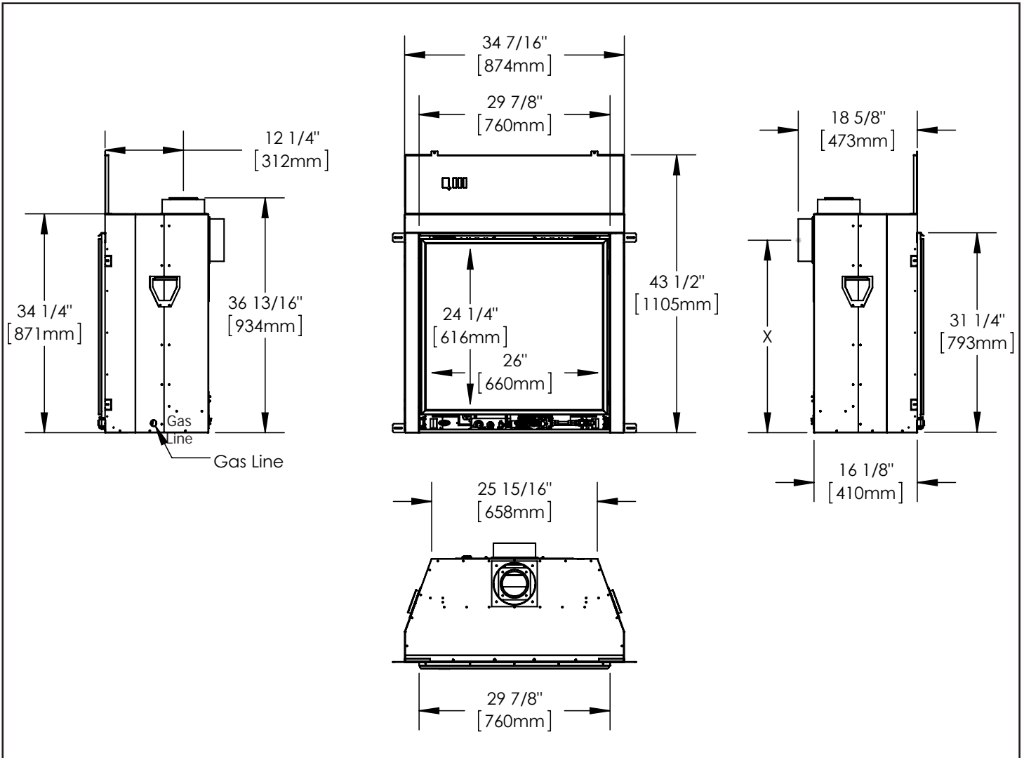
Figure 2. Q3 Dimensions
