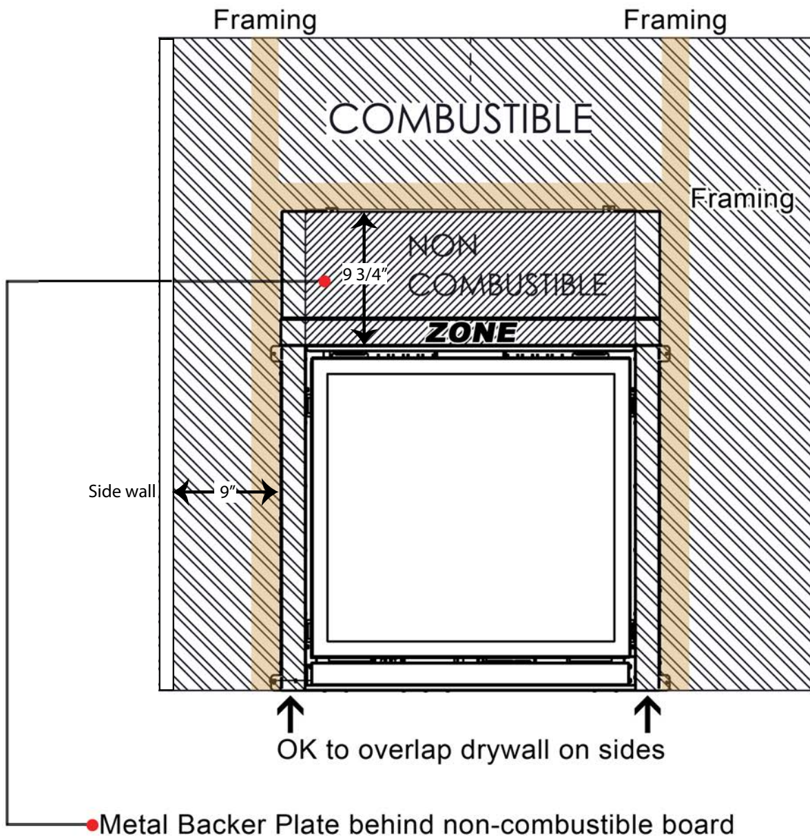
Figure 19: Non-Combustible Zone
